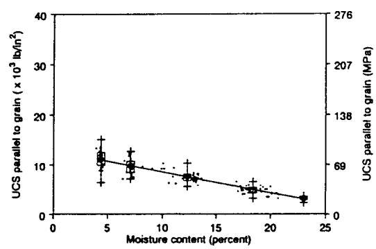
FIG. 12. Relationship of ultimate compressive stress (UCS) parallel-to-grain and moisture content.
