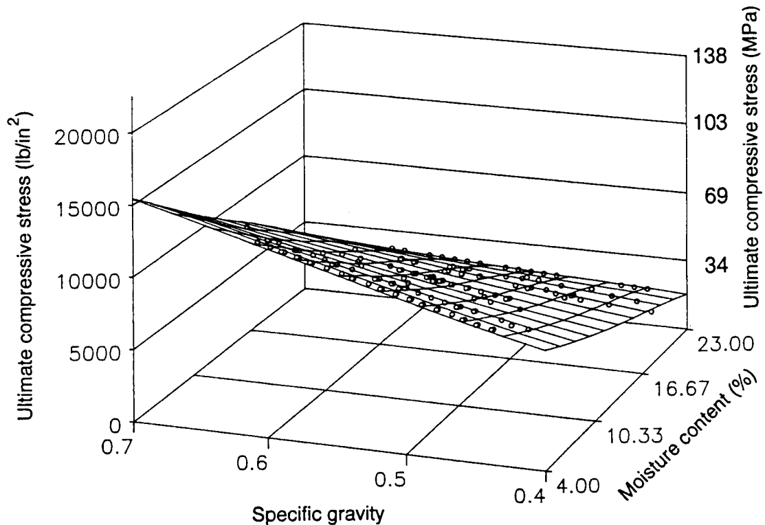
FIG. 19. Response surface for compression parallel-to-grain stress. Dots on surface represent x-y location of test data on surface.
