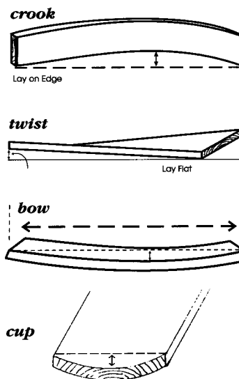
Figure 5.—Various kinds of warp.
