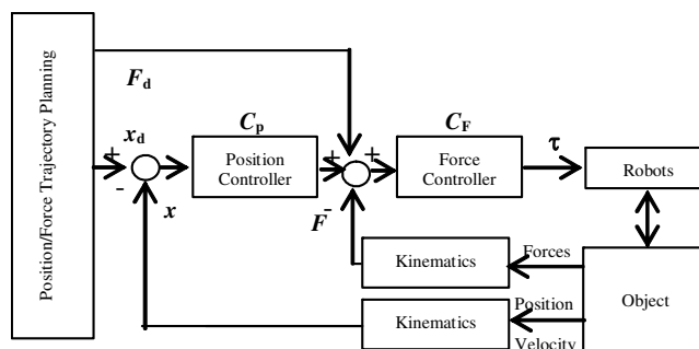
Figure 15: The position/force cascade controller.
